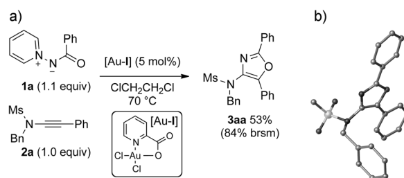
Scheme 1. a) Formal cycloaddition of ynamide 2a with the robust 1,3-N,O-dipole equivalent 1a . b) Crystal structure of 3aa ; hydrogen atoms omitted for clarity. Bn = benzyl, brsm = based on recovered starting material, Ms = methanesulfonyl.
